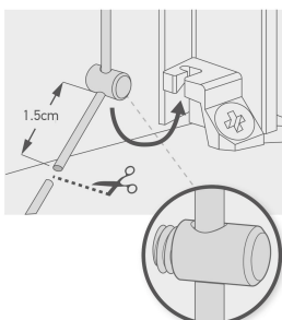
Fig 8A: Cord stop
